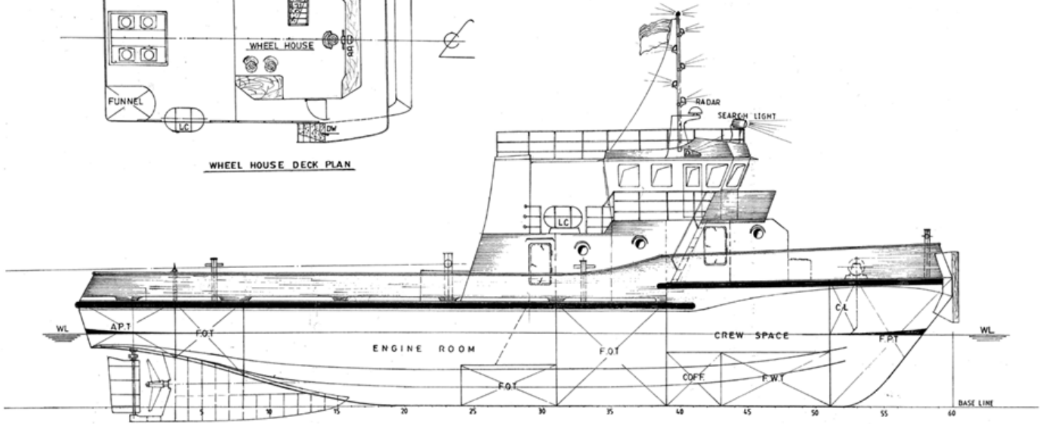
OUTBOARD PROFILE
