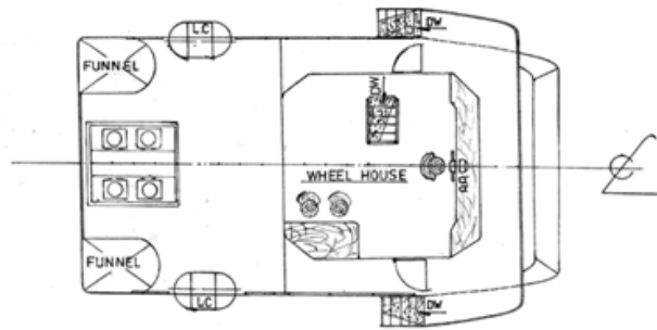
WHEEL HOUSE DECK PLAN
