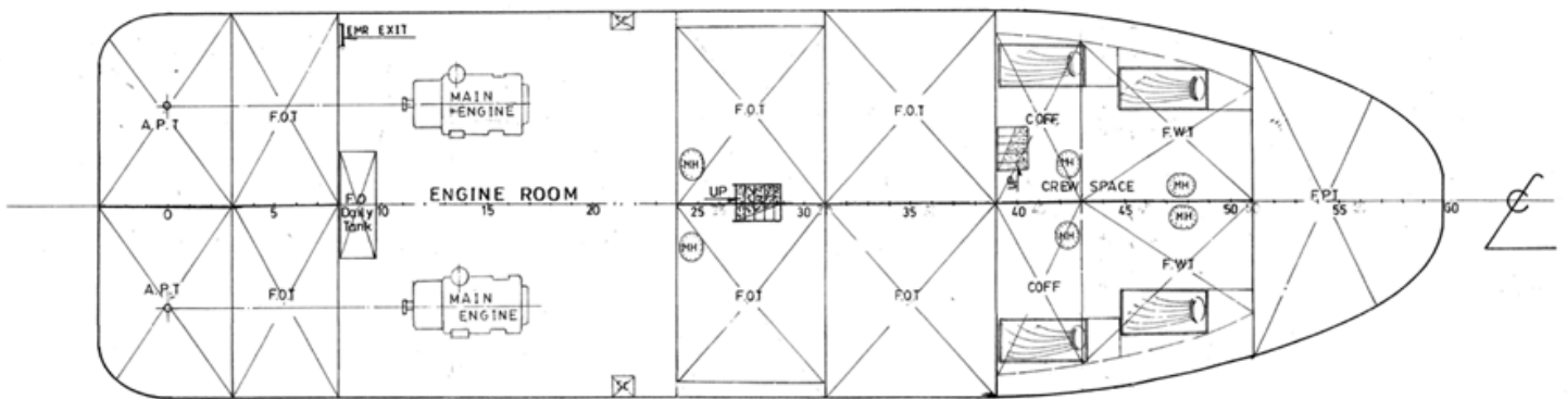
BELOW DECK PLAN
