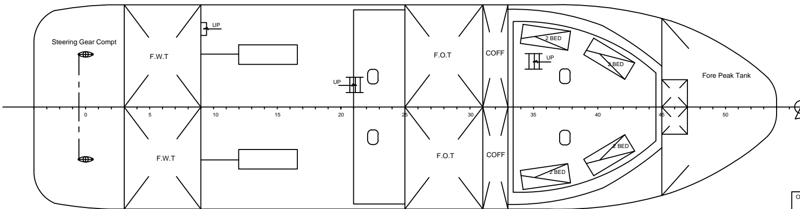
PLAN BELOW MAIN DECK
